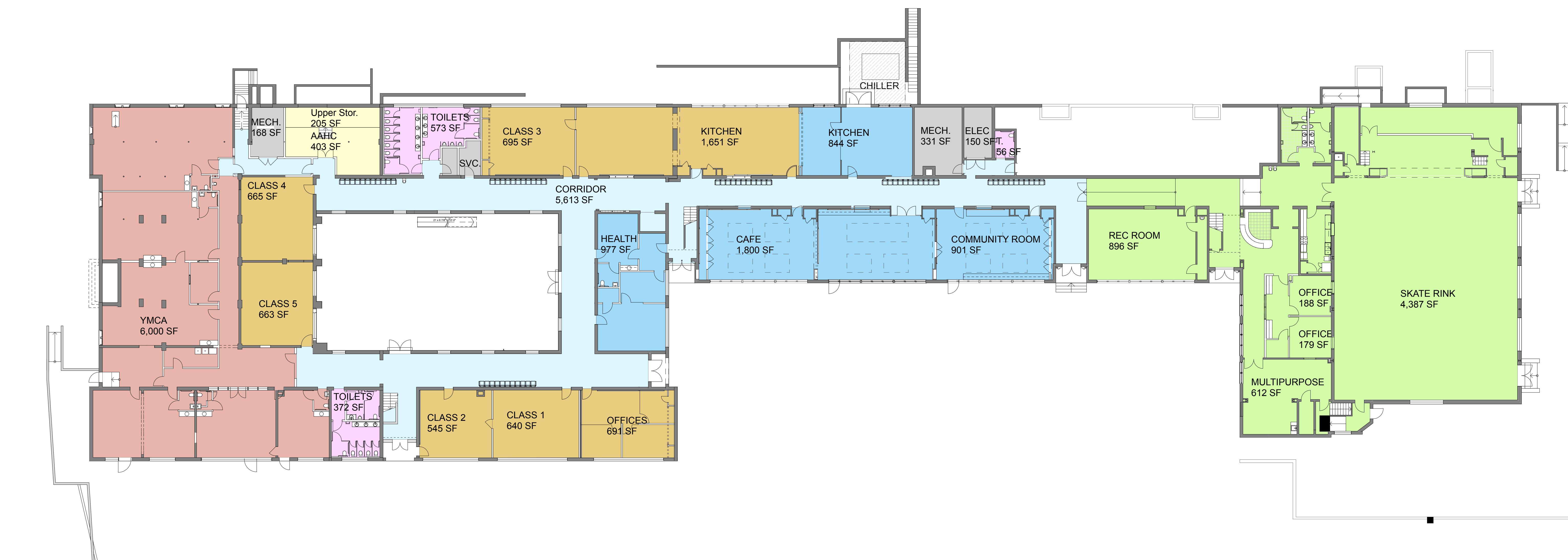
LOWER FLOOR PLAN
